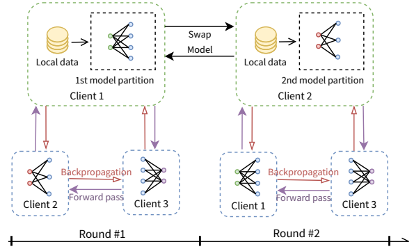
Fig. 3. In the case where multiple clients train with their local data and without aggregation, an exchange of model partitions between clients would be necessary if we need to minimize the use of GPU memory on the clients.
